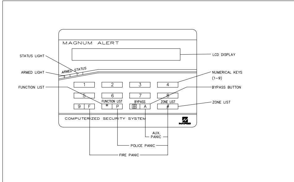
Keypad controls.
